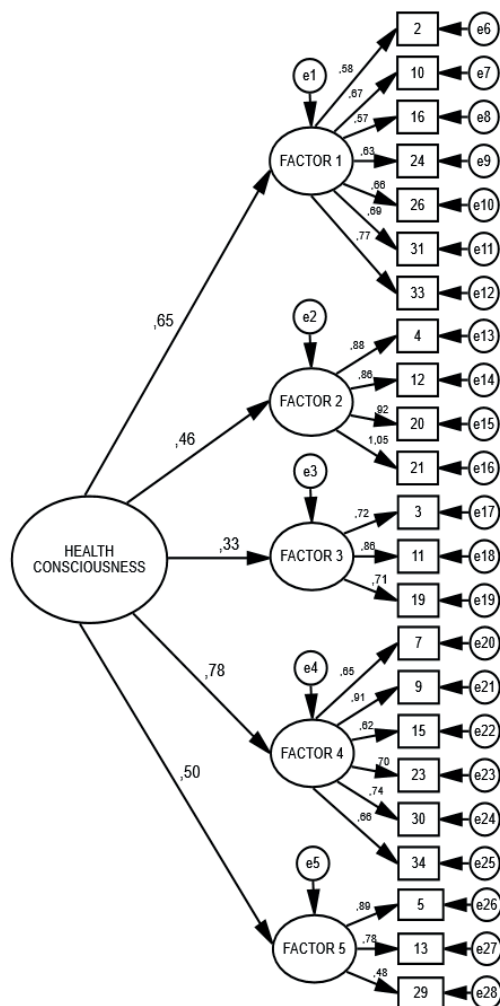
Fig. 1. Confirmatory factor analysis with standard estimation
