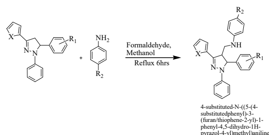
Figure 1. Scheme for synthesis of 4-substituted N-[(5-(4-substituted aryl)-3-heteroaryl-N1-phenyl-2-pyrazolines-4-yl)methyl]aniline
