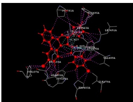
Figure 3. Binding interactions of 2b with cavity # 1 of 5I6X
