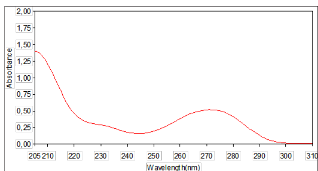
Figure 2. Absorption spectrum of caffeine in 0.1M HCl
