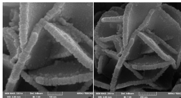
Figure 1. Scanning electron microscopy images of cellulose-magnesium oxide nanocomposite
